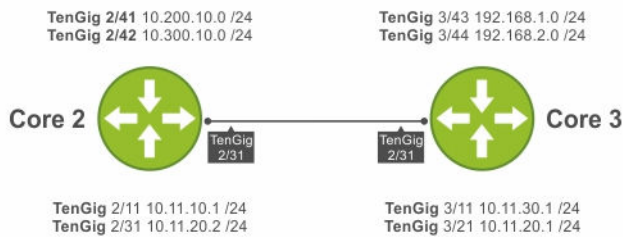
Figure 102. RIP Topology Example
